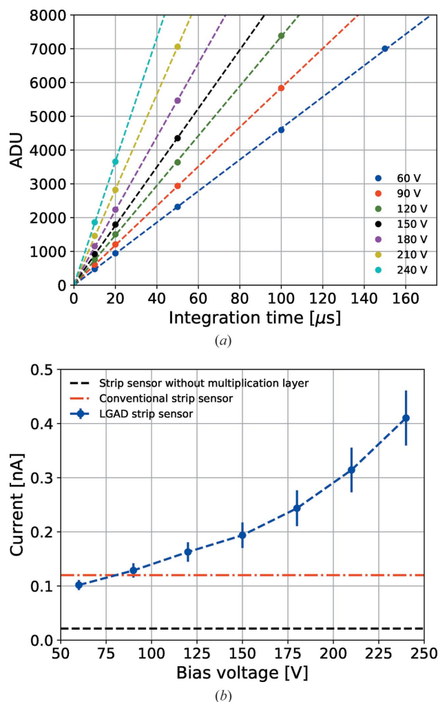
Figure 3 (a) Dynamic range scan using sensor leakage current for a single strip. (b) Average leakage current over all strips measured at different bias voltages compared with sensors without multiplication. The error bars represent the dispersion of the leakage current between the pixels.
