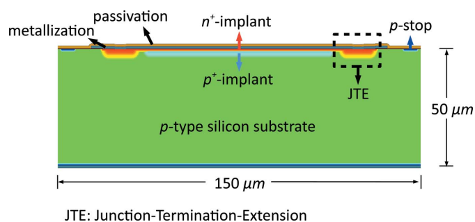
Figure 2 Cross section of the investigated LGAD sensors.
