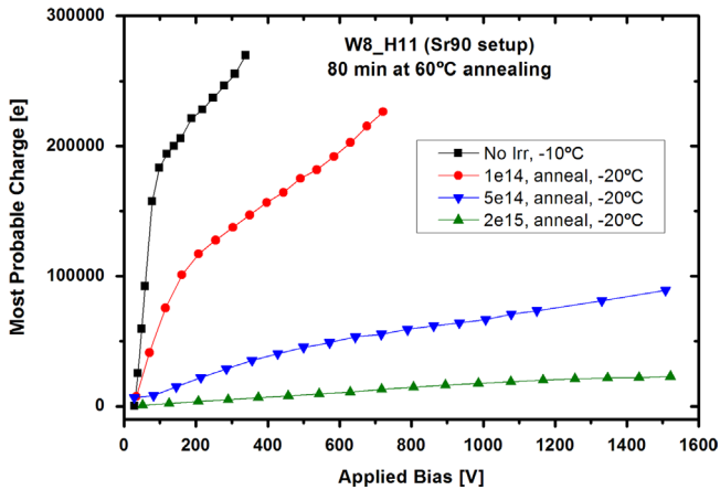
Fig. 10. Measured absolute collected charge as a function of the applied bias for a LGAD sample irradiated to different fluences.
