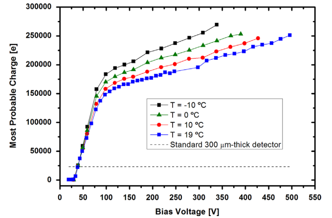
Fig. 9. Temperature dependence of the multiplication factor. Charge collection response for a MIP has been measured at different operational temperatures. The expected signal for a standard 300 \mu\text{m} -thick detector has been depicted with a dashed line to allow the comparison with a non-multiplying detector.
