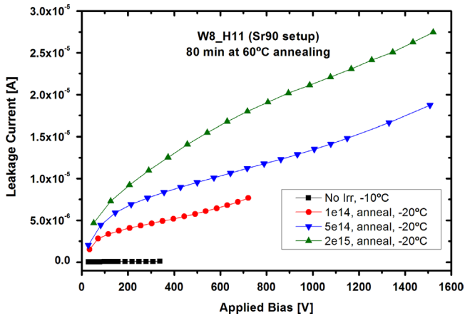
Fig. 11. Measured leakage current as a function of the applied bias for a LGAD sample irradiated to different fluences.
