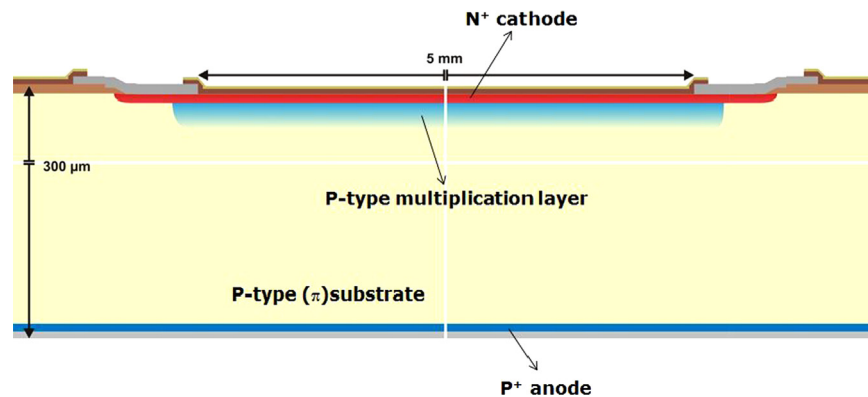
Fig. 1. Schematic cross-section of the LGAD pad design. A p-type layer is diffused below the n^+ electrode to form the n^+/p/p^- junction where the multiplication takes place.
