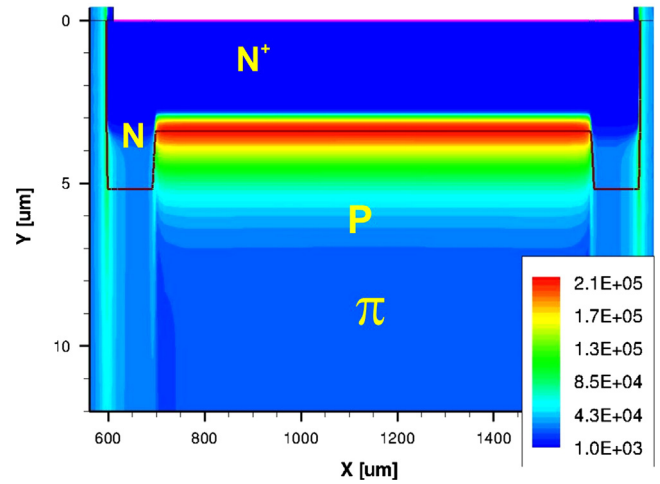
Fig. 5. Simulated electric field distribution throughout the multiplication junction of a LGAD ended with a JTE.
