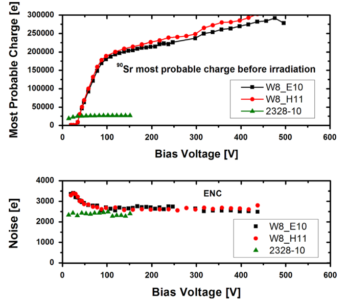
Fig. 8. Absolute collected charge (up) and noise (bottom) signals for two LGAD samples after Sr-90 source MIPs exposure. Measurements are compared with the response of a conventional non-multiplying pad diode (2328-10).
