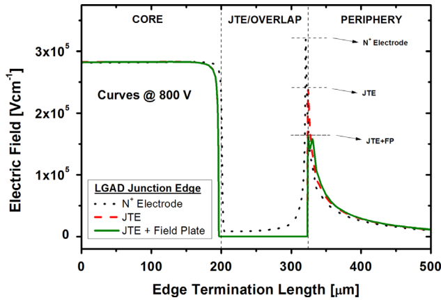
Fig. 3. Simulated electric field distribution at the multiplication junction edge for different termination designs: n + electrode extension, JTE, and JTE with field plate.
