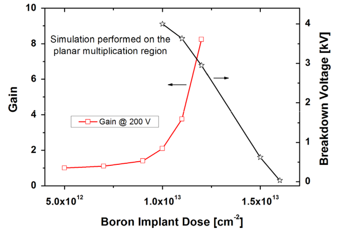
Fig. 2. Simulated dependence of gain and breakdown voltage as a function of the boron dose implanted to form the p well.
