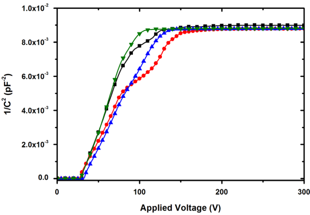
Fig. 7. 1/C^2 - V curves for a sampling of the fabricated devices. Each curve corresponds to similar samples located on the same wafer with boron implant dose = 1.6 \times 10^{13} \text{ cm}^{-2} .
