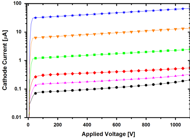
Fig. 6. I - V curves for a sampling of the fabricated device. Each curve corresponds to similar samples located on the same wafer with boron implant dose = 1.6 \times 10^{13} \text{ cm}^{-2} , can be grouped in three ranges, according to their current levels: I < 1 \mu\text{A} ; 1 \mu\text{A} < I < 10 \mu\text{A} ; and I > 10 \mu\text{A} . Voltage capability beyond 1100 V has been shown in all cases.
